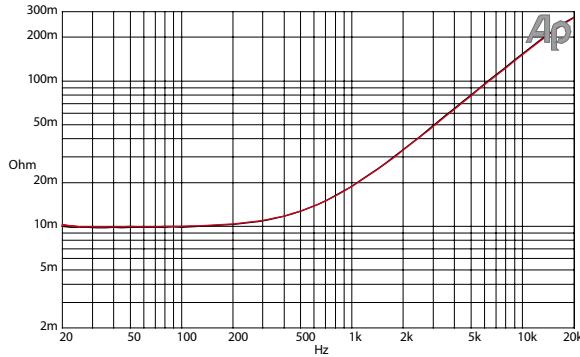
Figure 8.5 Output impedance vs. frequency @ 1 Amp RMS injected current (Ch1, Ch2) equivalent 11 m \Omega + 2,1 \mu H (Measurements of a typical performance of TECTON 32.4 )
