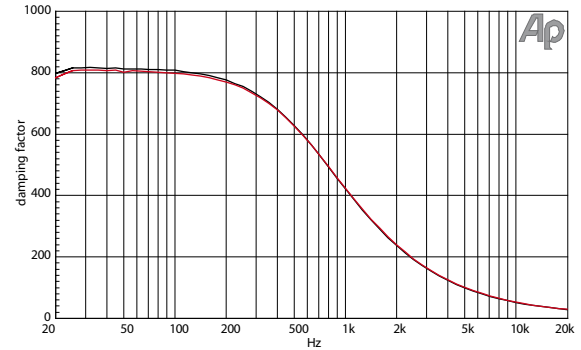
Figure 8.7 Damping factor into 8 \Omega (Ch1, Ch2) equation: damping factor = loaded impedance / amplifier output impedance (Measurements of a typical performance of TECTON 32.4 )
