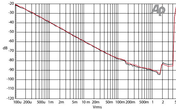
Figure 8.6 THD+N @ 1 kHz, 8 \Omega load vs. input voltage (Ch1, Ch2) (Measurements of a typical performance of TECTON 32.4 )
