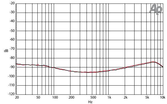
Figure 8.8 THD+N vs. frequency (BW 22 kHz), 10 dB below clip, 8 \Omega (Ch1, Ch2) (Measurements of a typical performance of TECTON 32.4 )
